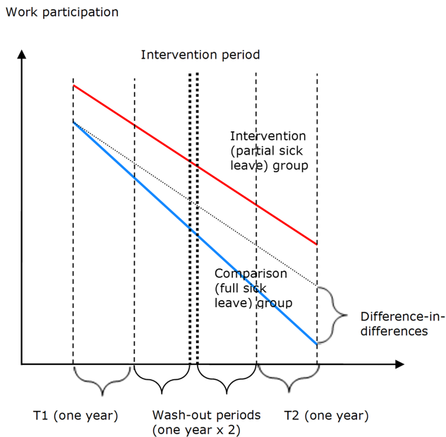
Figure 1 Schematic presentation of the study design and difference-in-differences method. (T1 corresponds to preintervention period, T2 corresponds to postintervention period).
